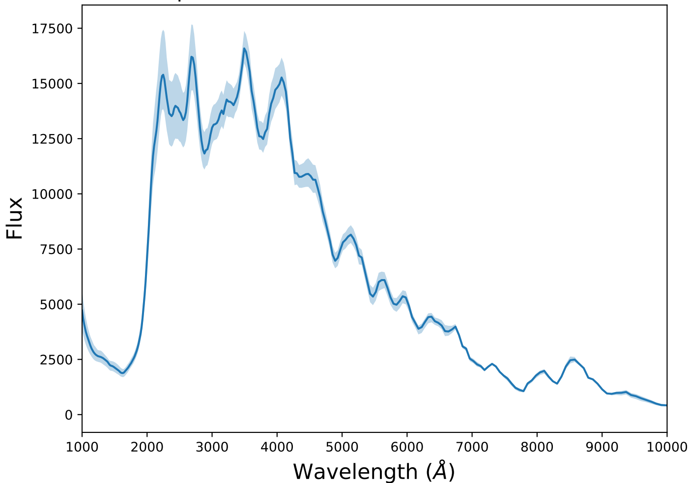
Spectrum 8 for transient SNIa at z=0.31
